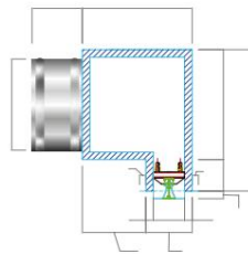
Detail PS2F height 50 mm with S connection
